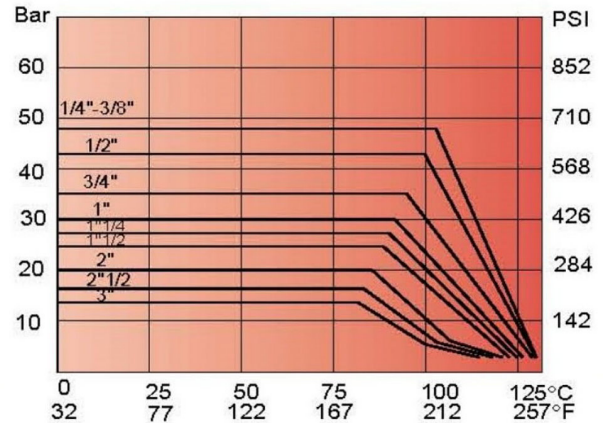
PRESSURE/TEMPERATURE DIAGRAM
