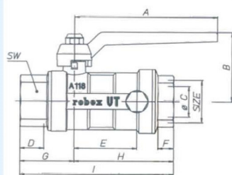
Art. S.370 ROBEX.VT Triple valve with aluminium lever, female/female.
