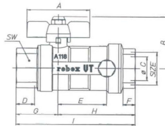
Art. S.380 ROBEX.VT Triple valve with T-handle, female/female
